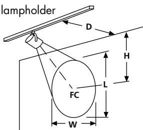
Figure 1 Single lampholder
